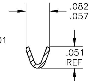
SECTION A-A SCALE 8:1
