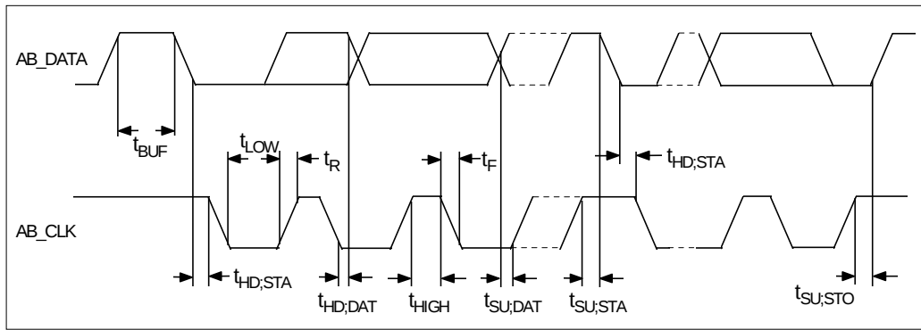
FIGURE 46 - ACCESS.bus TIMING
