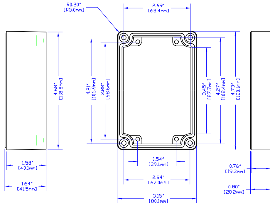
VIEW OF LID (INSIDE)
