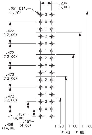
PC MOUNTING
