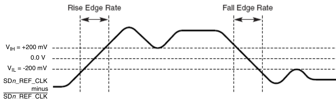
Figure 52. Differential Measurement Points for Rise and Fall Time
