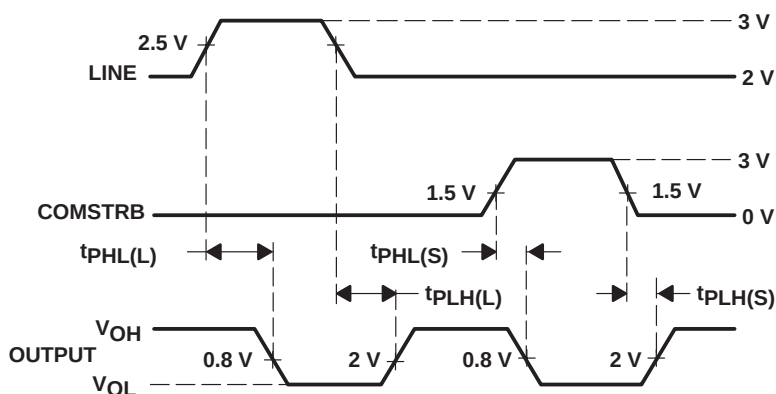
VOLTAGE WAVEFORMS
