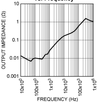
MIC2930x Output Impedance vs. Frequency
