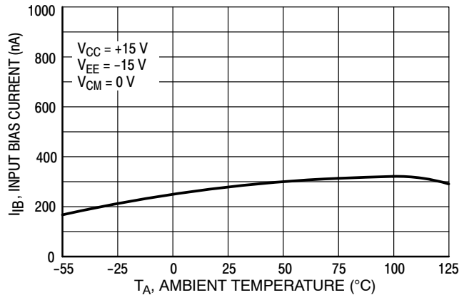
Figure 2. Input Bias Current versus Temperature
