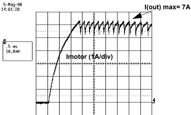
Figure 17. Current Limitation
