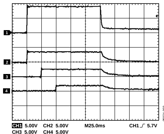
Figure 2. Sequenced Waveforms
