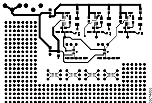
Figure 5. Component-Side Silkscreen
