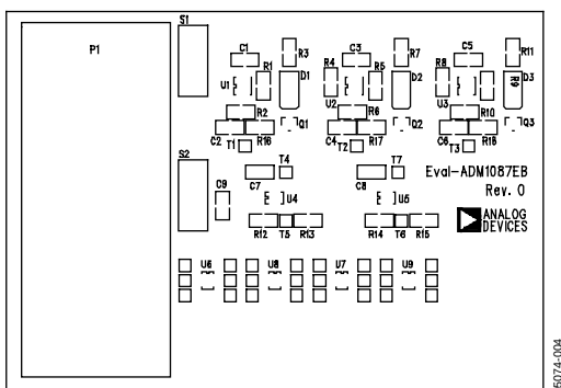
Figure 4. Evaluation Board Layout
