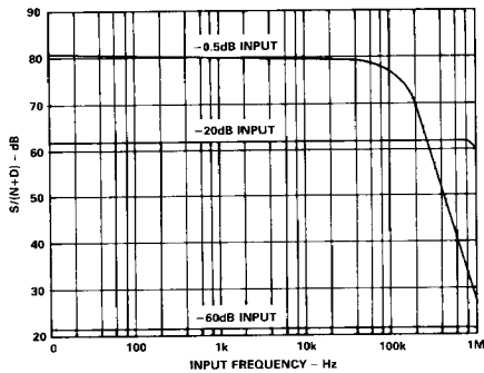
Figure 15. S/(N+D) vs. Input Frequency and Amplitude
