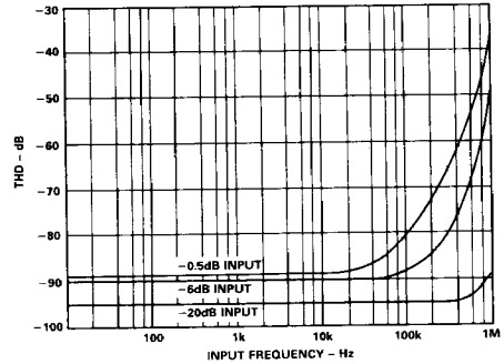
Figure 14. Total Harmonic Distortion vs. Input Frequency and Amplitude
