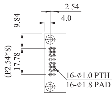
PIN DETAIL
