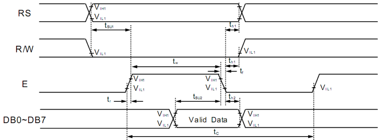
Writing data from MPU to KS0066U
