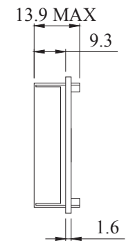
LED B/L
