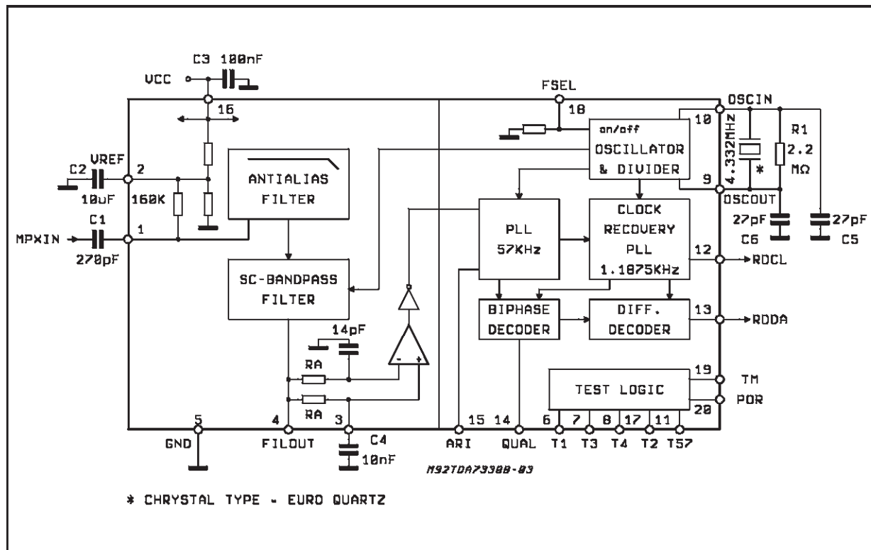
Figure 3: Test Circuit
