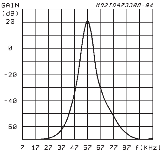
Figure 5: Gain vs. Frequency
