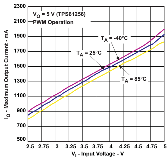
Figure 12. Maximum Output Current vs Input Voltage
