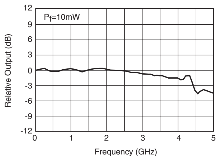
Fig. 2 Frequency Response
