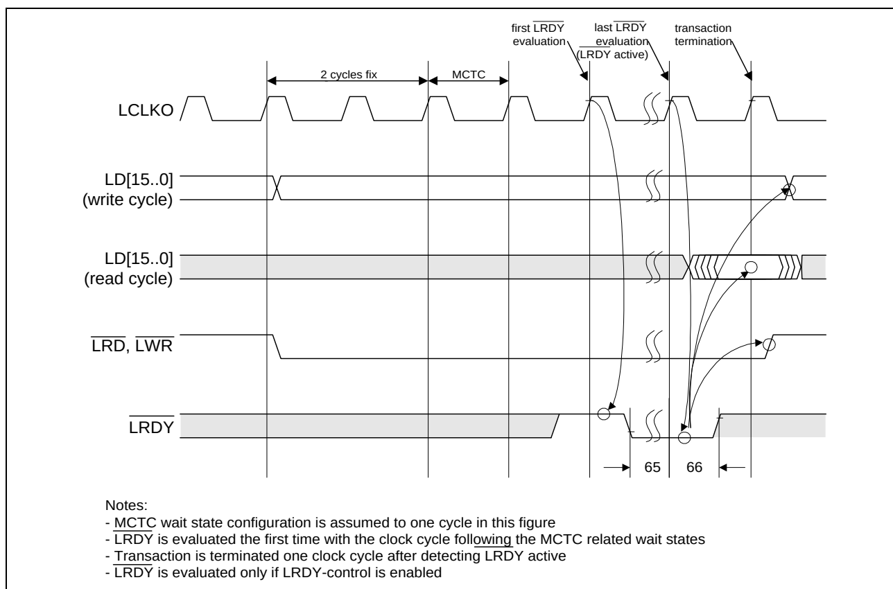
Figure 97 LRDY Timing
