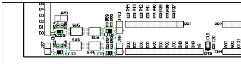
Figure 5.15 User LEDs
