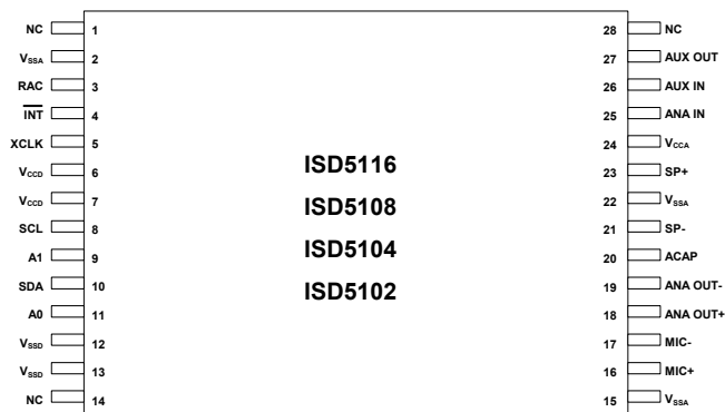
TSOP
