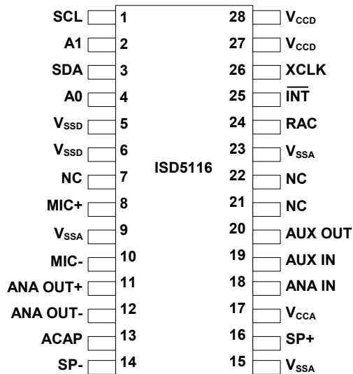
PDIP
