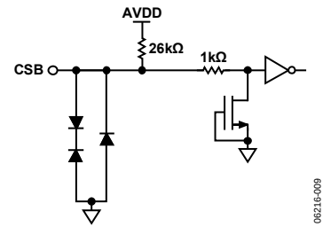
Figure 9. Equivalent CSB Input Circuit
