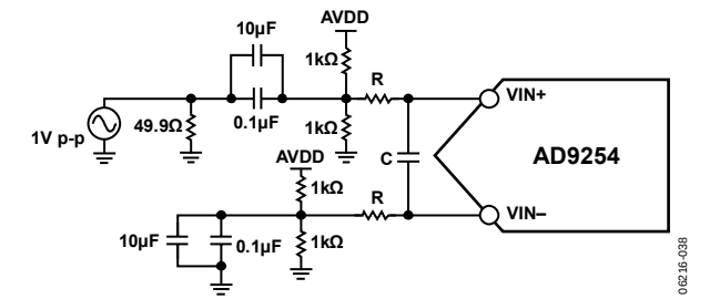
Figure 34. Single-Ended Input Configuration
