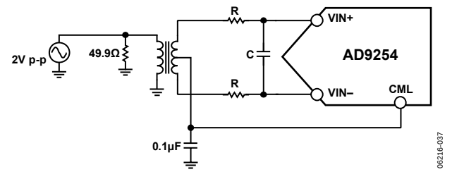
Figure 33. Differential Transformer-Coupled Configuration
