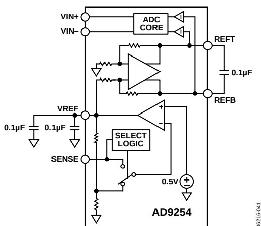
Figure 37. Internal Reference Configuration
