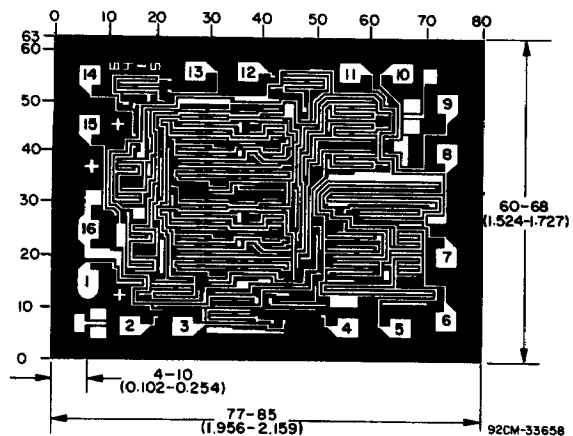
Dimensions and pad layout for CD4063BH.
