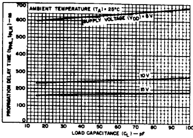
Fig. 7 - Typical propagation delay time vs. load capacitance ("comparing inputs" to outputs).
