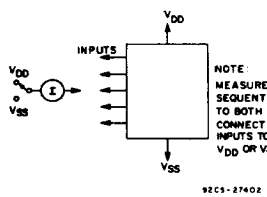
Fig. 11 - Input current test circuit.
