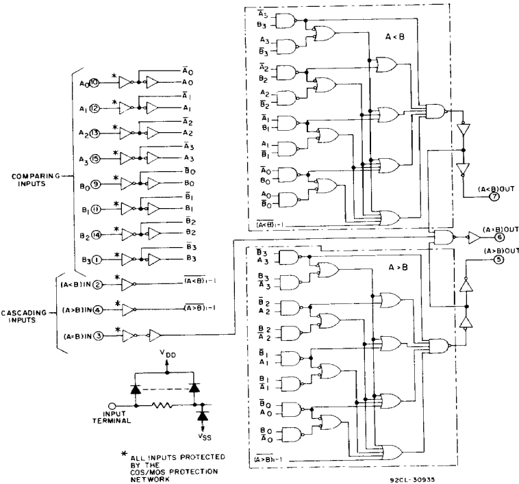
Fig. 2 -- Logic diagram for CD4063B.
