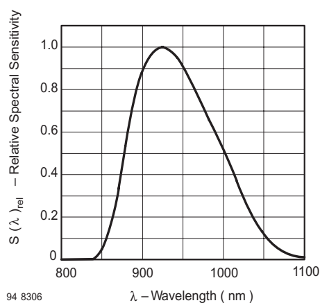
Figure 8. Relative Spectral Sensitivity vs. Wavelength
