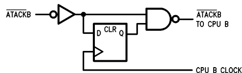
C. Synchronize \overline{\text{ATACKB}} to CPU B Clock. This is useful if CPU B runs asynchronous to the DP8422.
