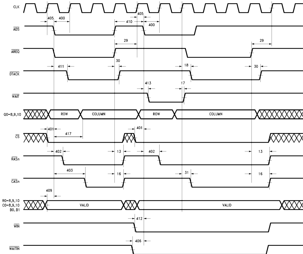
FIGURE 42. 400: Mode 1 Timing
