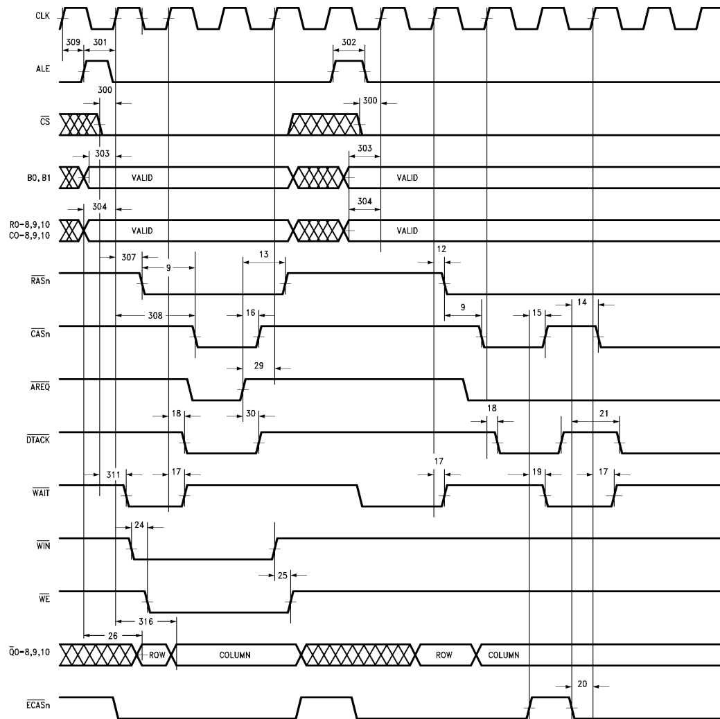
FIGURE 40. 300: Mode 0 Timing
