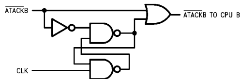
A. Extend \overline{\text{ATACKB}} to 1/2T ( 1/2 Clock) after \overline{\text{RAS}} goes low.
