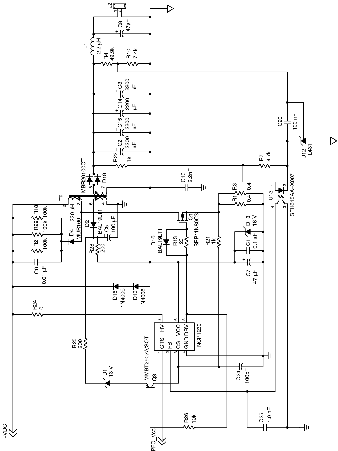
Figure 11. DC-DC section
