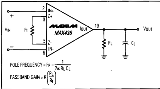
Figure 8. Lowpass Amplifier
