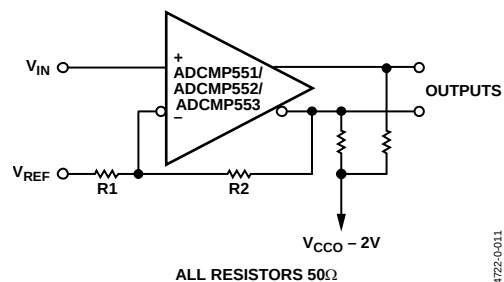
Figure 22. Hysteresis Using Positive Feedback
