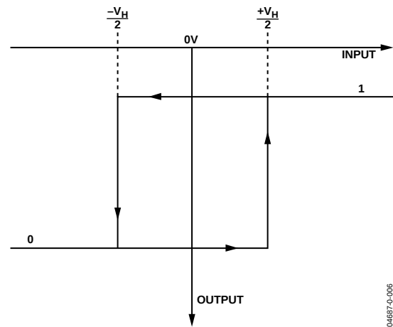
Figure 18. Comparator Hysteresis Transfer Function
