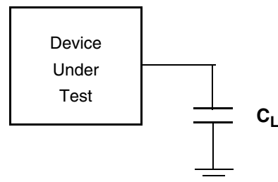
Figure 6.3 Test Setup
