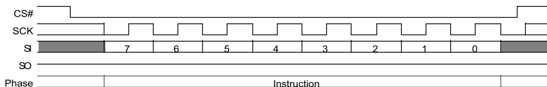
Figure 10.67 PPB Erase (PPBE E4h) Command Sequence
