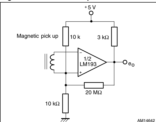
Figure 13. Transducer amplifier
