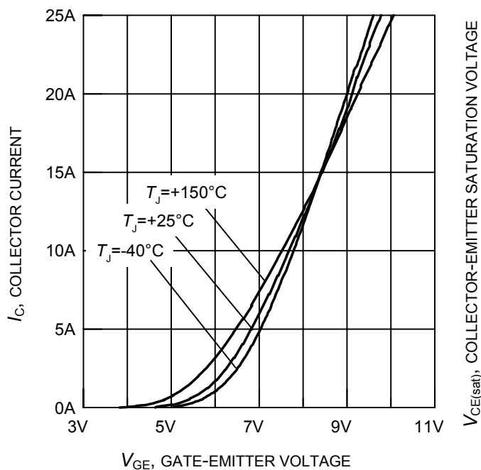
Figure 7. Typical transfer characteristics ( V_{CE} = 20\text{V} )
