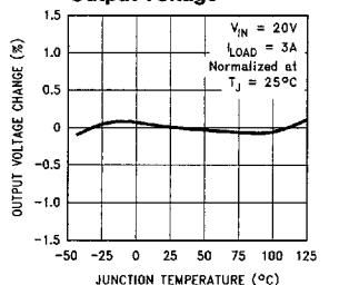
Normalized Output Voltage
