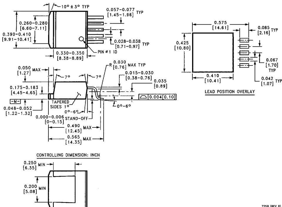
5-Lead TO-263 Surface Mount Package (S) Order Number LM2596S-3.3, LM2596S-5.0, LM2596S-12 or LM2596S-ADJ NS Package Number TSSB
