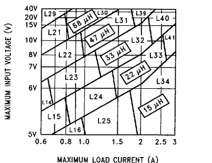
FIGURE 5. LM2596-3.3
