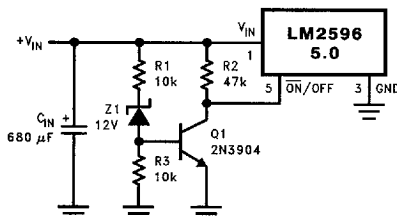
FIGURE 22. Undervoltage Lockout for Buck Regulator
