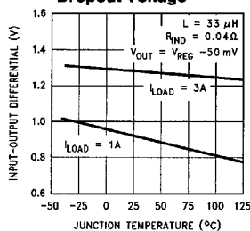
Dropout Voltage
