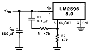
FIGURE 21. Delayed Startup
