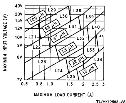
FIGURE 6. LM2596-5.0
