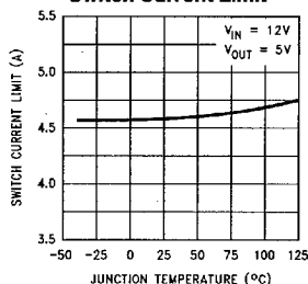
Switch Current Limit
