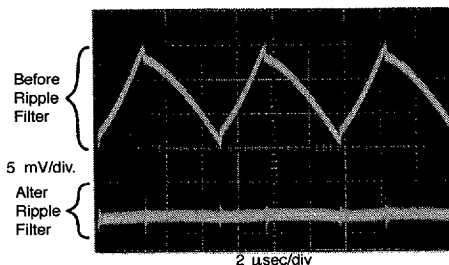
FIGURE 17. Post Ripple Filter Waveform
