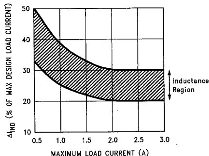
FIGURE 16. ( \Delta I_L ) Peak-to-Peak Inductor Ripple Current (as a Percentage of the Load Current) vs Load Current
