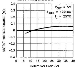
Line Regulation
