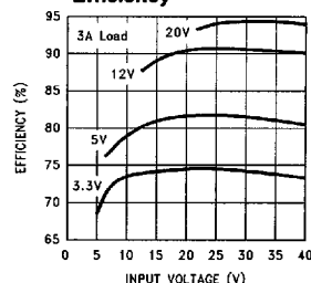
Efficiency
