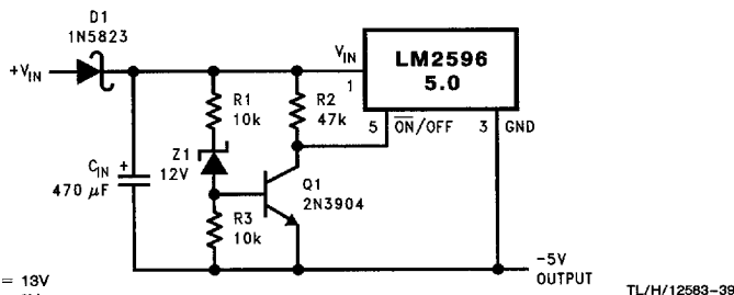
FIGURE 24. Undervoltage Lockout with Hysteresis for Inverting Regulator
