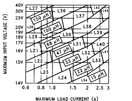
FIGURE 7. LM2596-12
