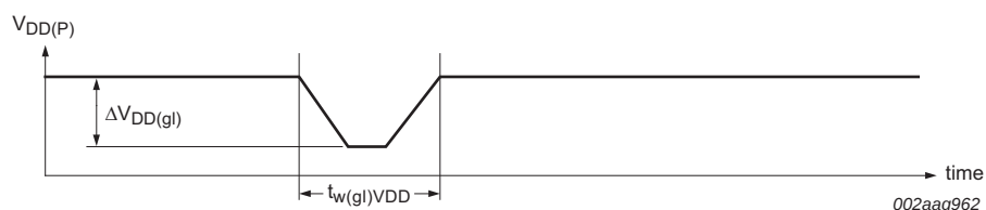
Fig 19. Glitch width and glitch height
