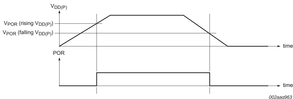
Fig 20. Power-on reset voltage ( V_{POR} )
