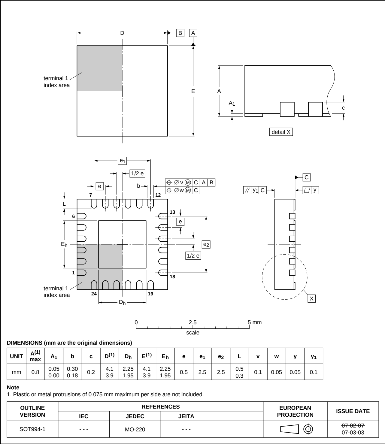
Fig 32. Package outline SOT994-1 (HWQFN24)
