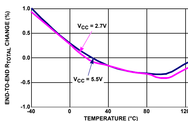
FIGURE 16. END-TO-END R_{TOTAL} % CHANGE vs TEMPERATURE, 50k (U)
