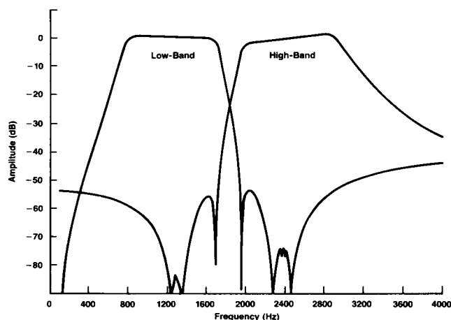
FIGURE 2. LOW-BAND AND HIGH-BAND AMPLITUDE RESPONSE - NORMALIZED
