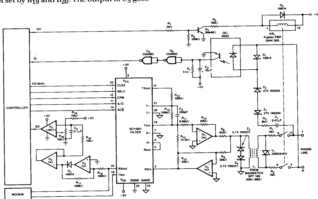
FIGURE 16. A CALL PROGRESS MONITORING APPLICATION
