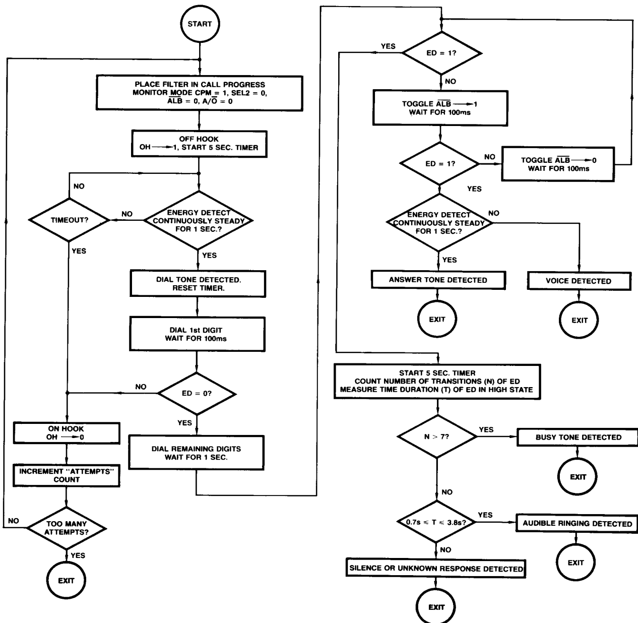
FIGURE 17. CALL PROGRESS MONITORING ALGORITHM
