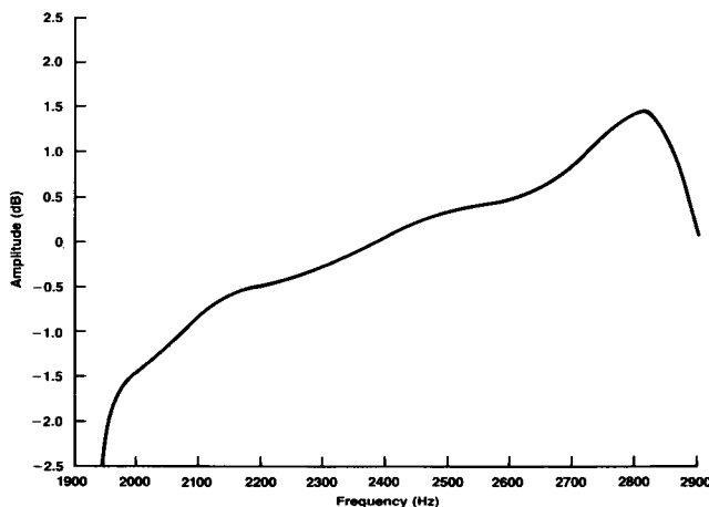
FIGURE 5. HIGH-BAND RESPONSE - NORMALIZED
