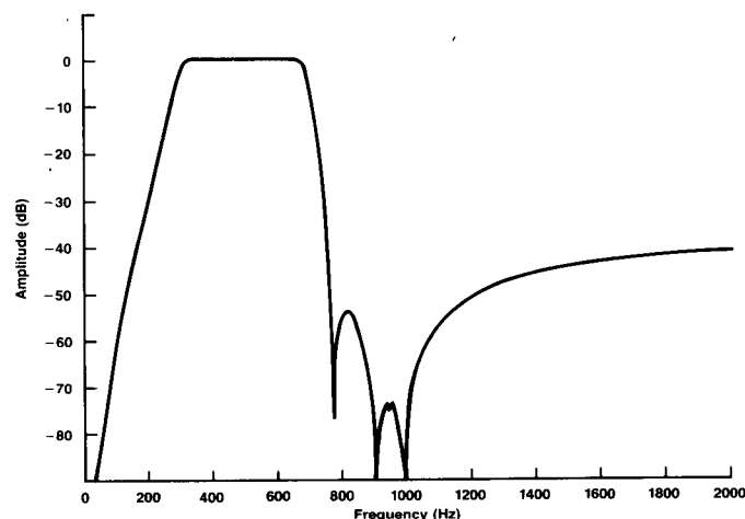
FIGURE 7. LOW-BAND DIVIDED BY 2.5 AMPLITUDE RESPONSE – NORMALIZED
