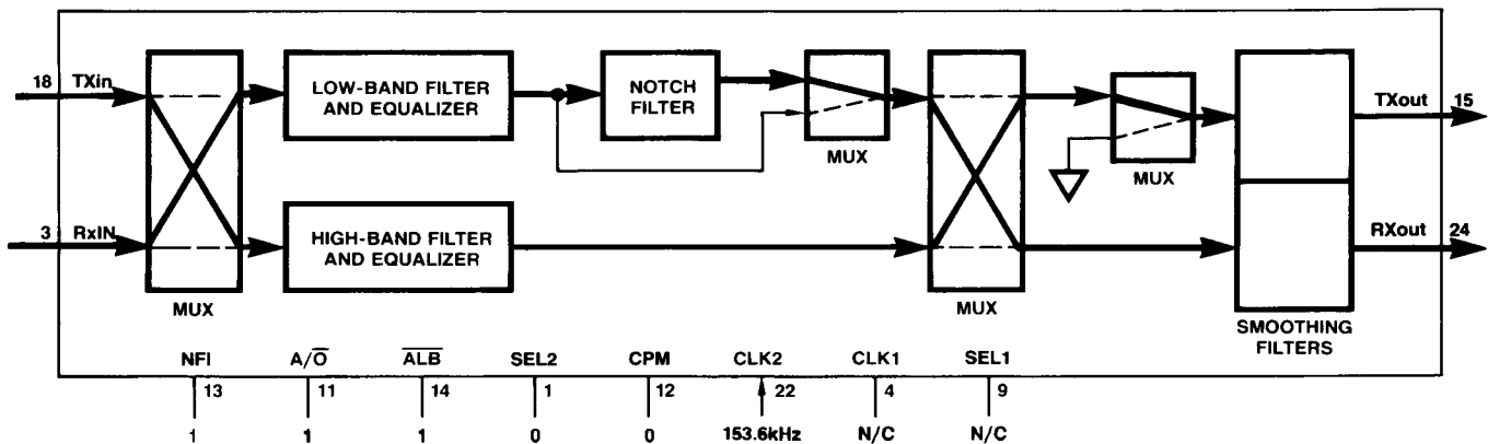
FIGURE 10. V.22 ANSWER MODE
