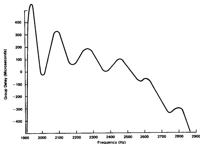
FIGURE 6. HIGH-BAND GROUP DELAY (Hz)
