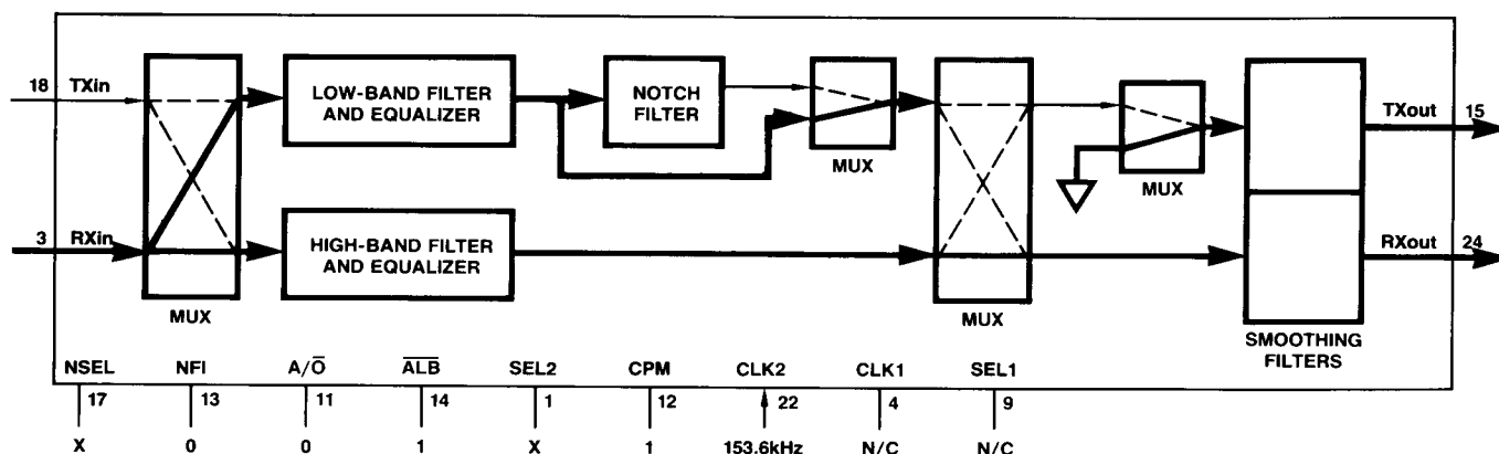
FIGURE 14. CALL PROGRESS MONITOR MODE: MONITORING ANSWER TONE/VOICE
