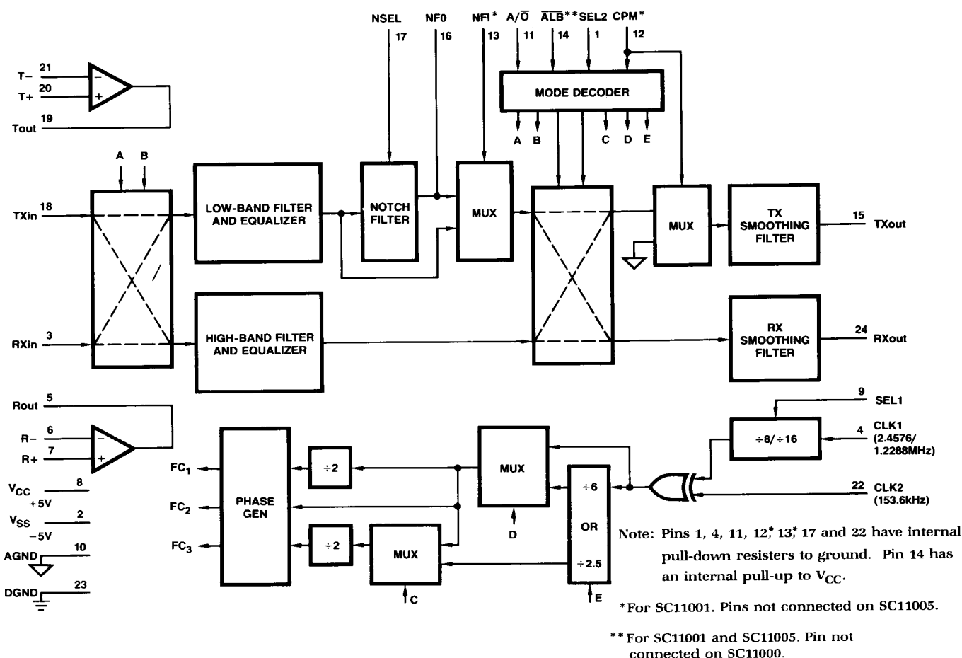
FIGURE 1. SC11000/SC11001/SC11005 MODEM FILTER BLOCK DIAGRAM
