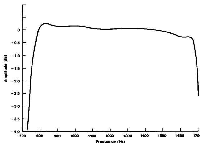
FIGURE 3. LOW-BAND RESPONSE - NORMALIZED
