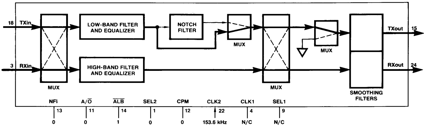
FIGURE 8. 212A ORIGINATE MODE
