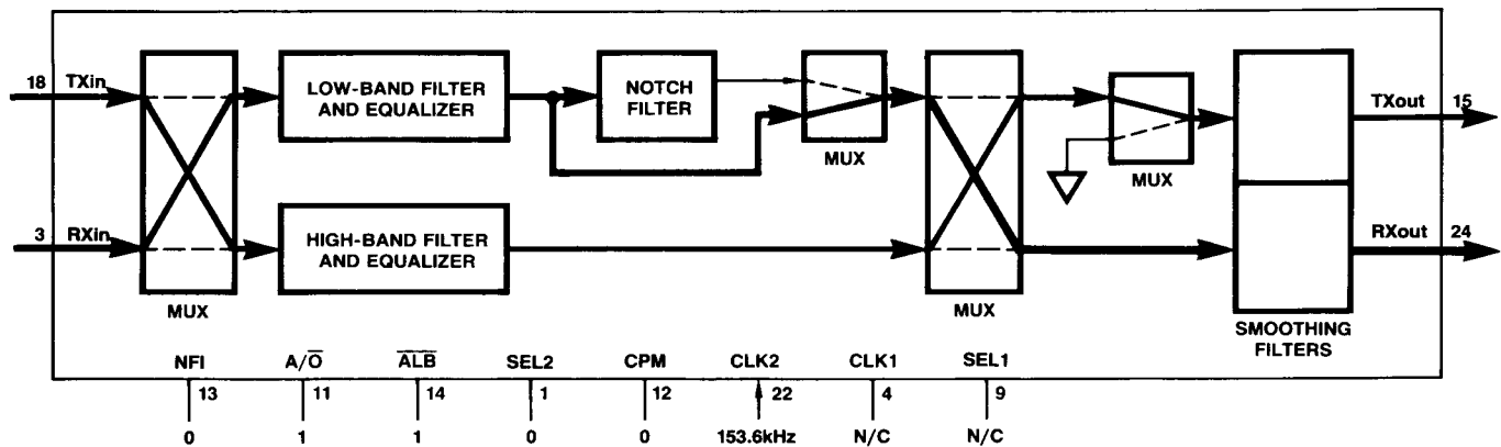
FIGURE 9. 212A ANSWER MODE
