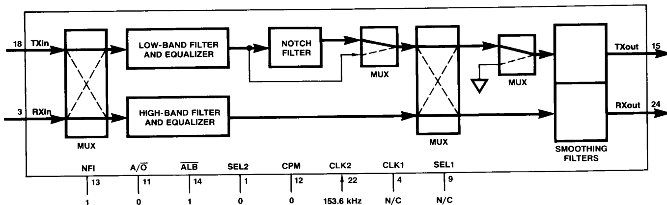
FIGURE 11. V.22 ORIGINATE MODE
