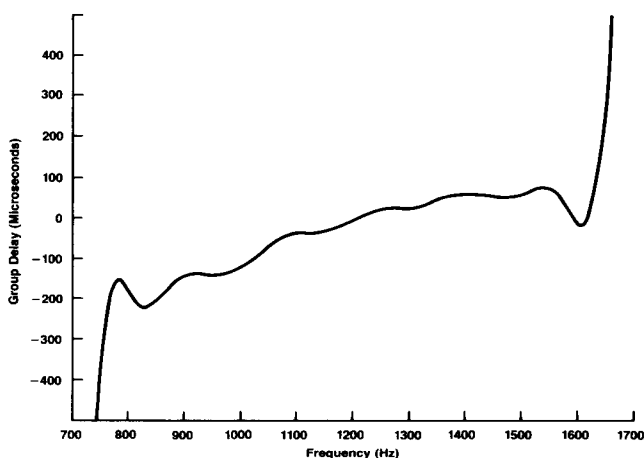
FIGURE 4. LOW-BAND GROUP DELAY
