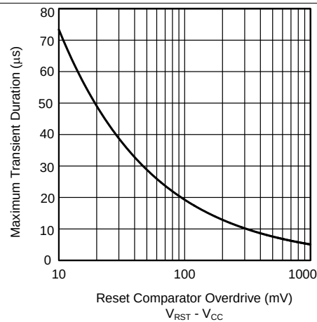
Figure 9. Maximum Transient Duration vs Reset Comparator Overdrive
