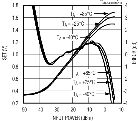
MAX4000 SET AND LOG CONFORMANCE vs. INPUT POWER AT 2.5GHz (UCSP)
