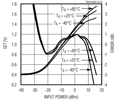
MAX4001 SET AND LOG CONFORMANCE vs. INPUT POWER AT 2.5GHz (UCSP)
