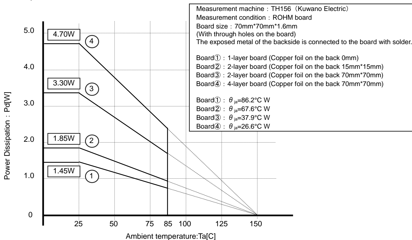
Fig.2 HTSSOP-B28 Thermal derating curve
