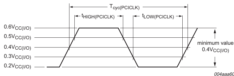
Fig 7. PCI clock.
