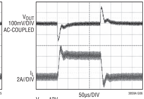
Load Step (Buck) Forced Continuous Mode
