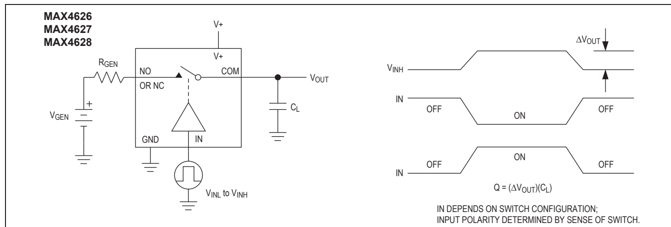
Figure 3. Charge Injection
