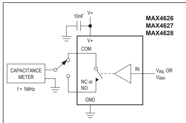
Figure 5. Channel Off/On-Capacitance
