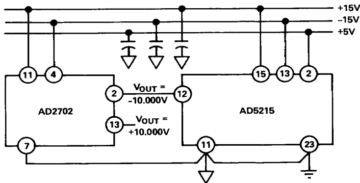
Using AD2702 Reference with the Fast, High Accuracy AD5215 – 12-Bit ADC
