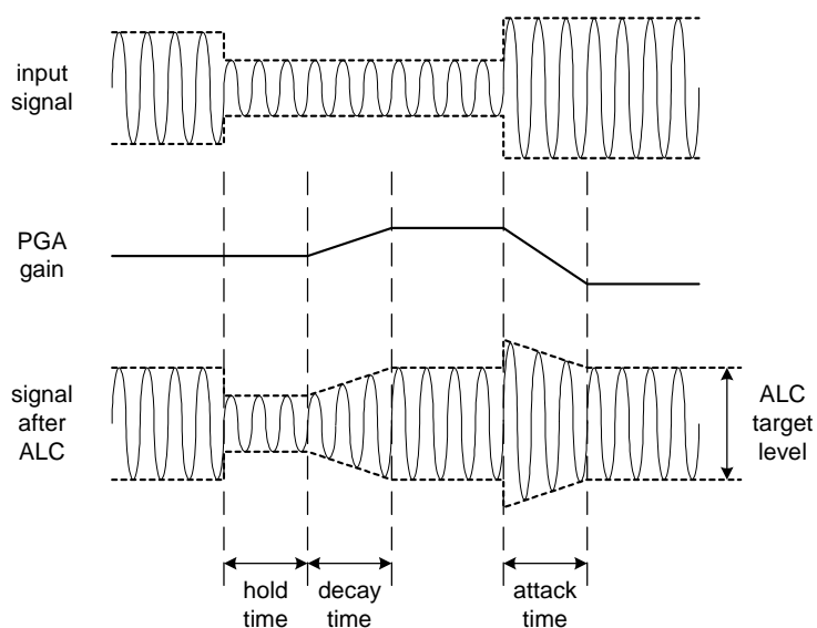
Figure 24 ALC Operation
