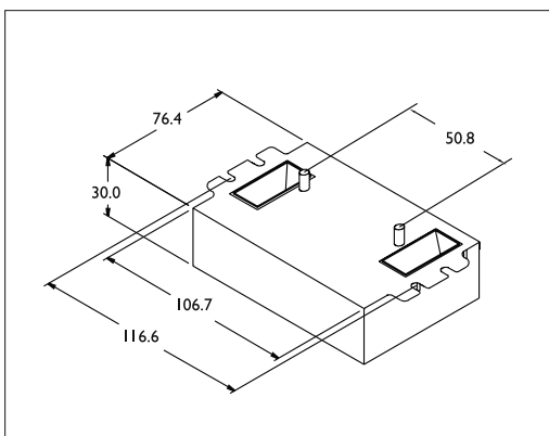
39W Driver
