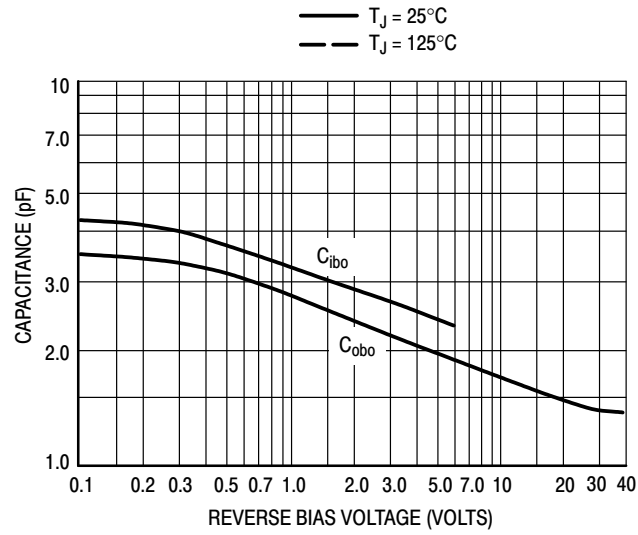
Figure 3. Capacitance
