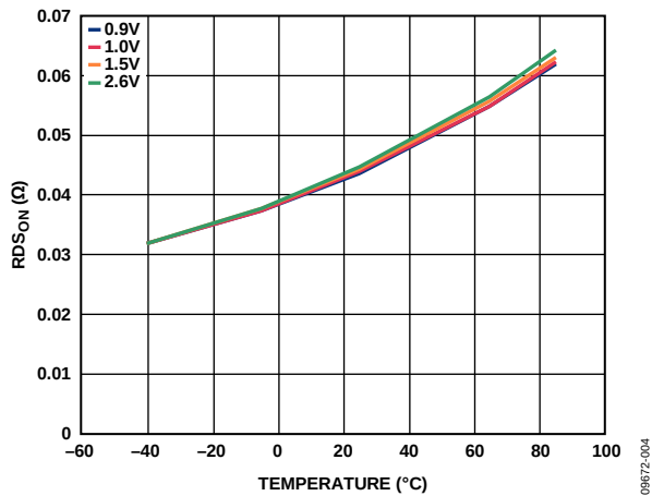
Figure 4. R_{DS(ON)} vs. Temperature, 50 mA, Different Input Voltage ( V_{IN} )
