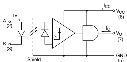
SFH6701, SFH6711
