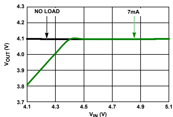
FIGURE 33. DROPOUT, ISL21080-41
