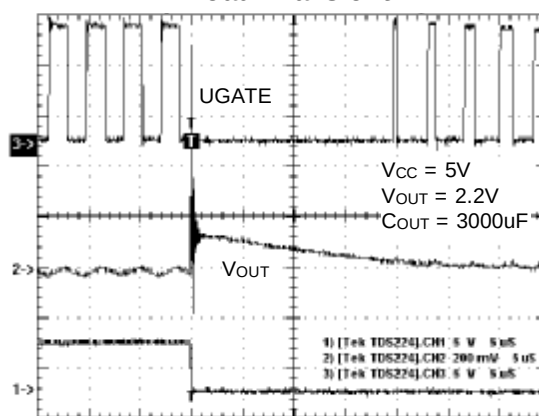
Load Transient
