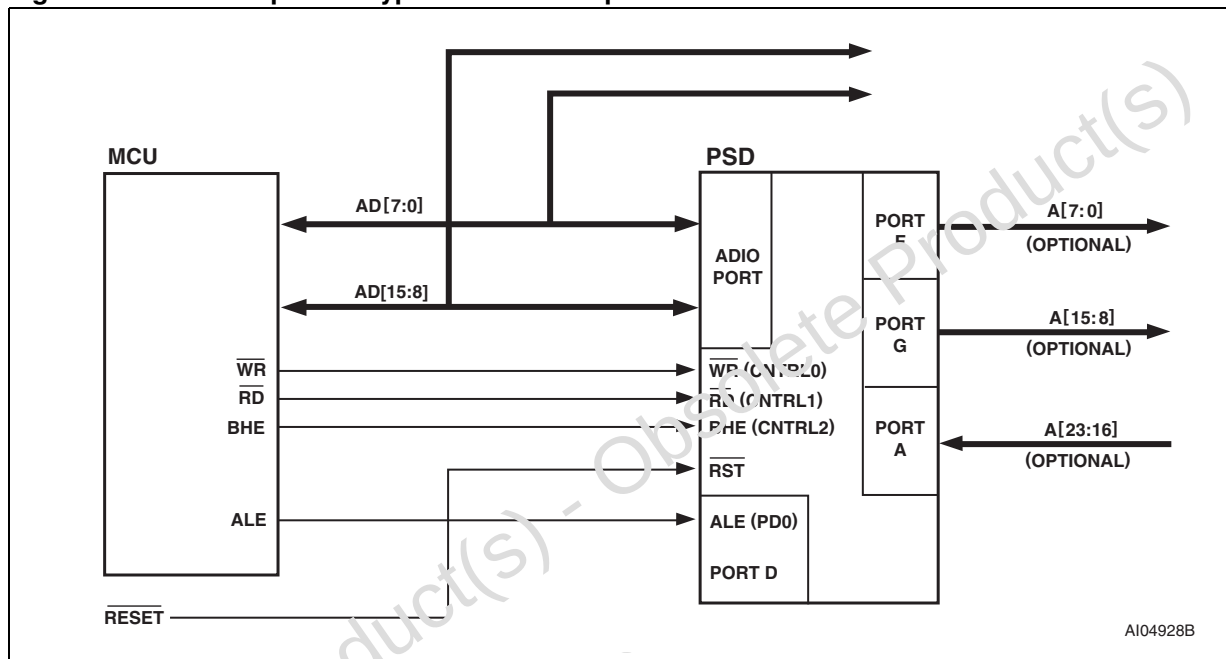
Figure 15. An example of a typical 16-bit multiplexed bus interface
