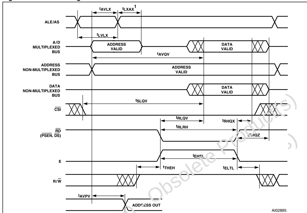
Figure 35. READ timing
