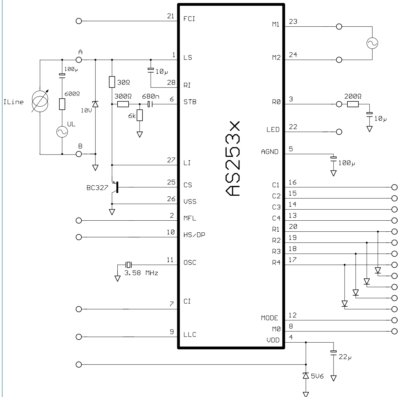
Figure 9 Test Circuit
