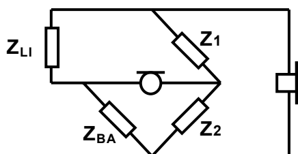
Figure 5 Side Tone Balance
