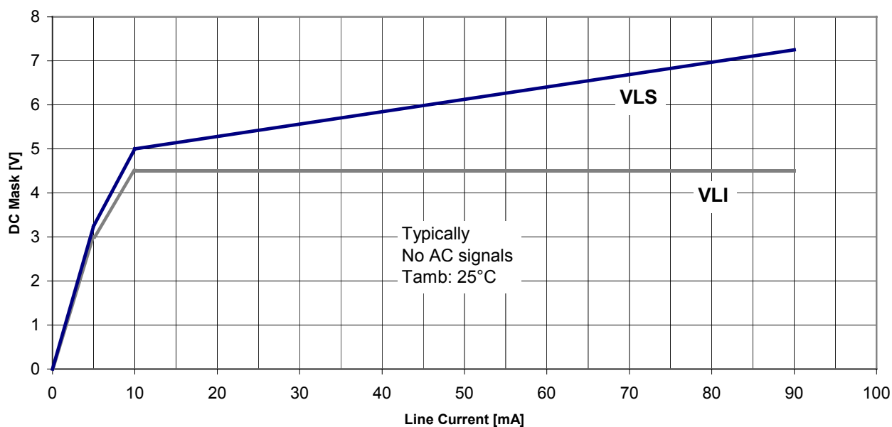
Figure 12 DC Mask
