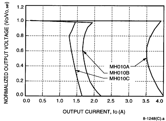
Figure 4. MH010A, B, C Typical Output Characteristics with V_i = 5\text{ V} , T_a = 25\text{ }^{\circ}\text{C}
