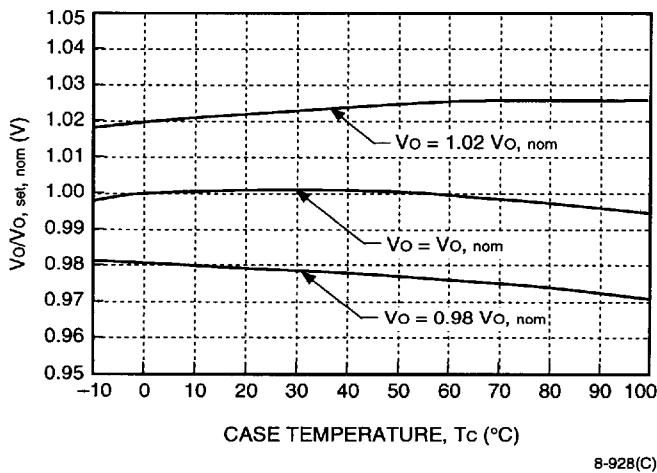
Figure 2. MH010-Series Typical Output Voltage Variation Over Operating Case Temperature
