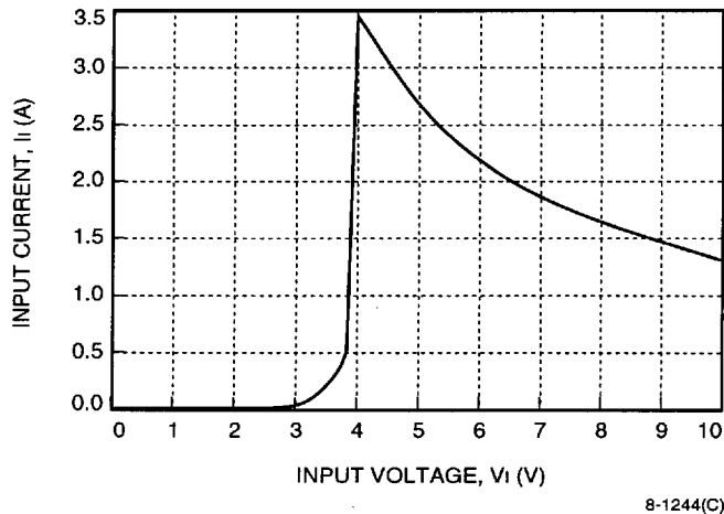
Figure 1. MH010-Series Typical Input Characteristic with I_o = I_{o,max} ; T_c = 25\text{ }^{\circ}\text{C}
