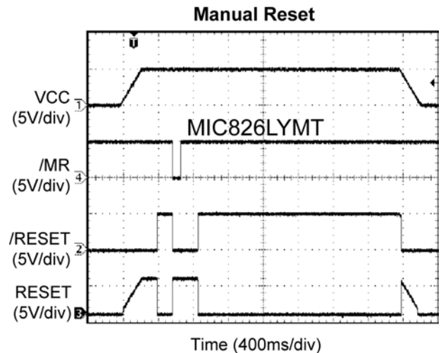
Figure 3. Manual Reset Function
